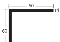
KP 88.543/60 x 60 x 4,0
