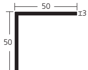
KP 80.578/50 x 50 x 3,0
