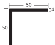
KP 80.579/50 x 50 x 4,0
