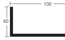
KP 89.547 /100 x 40 x 4,0
