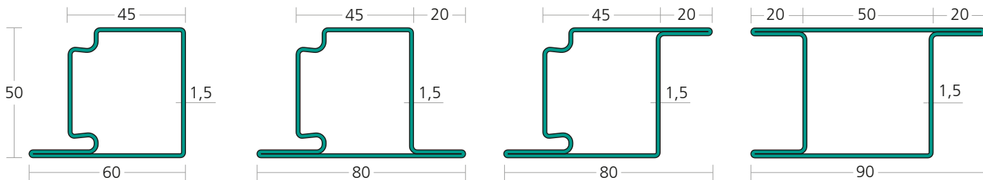
WP 950003 blank WP 951003 strip galvanized
