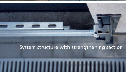
Individual constructions with additional post
