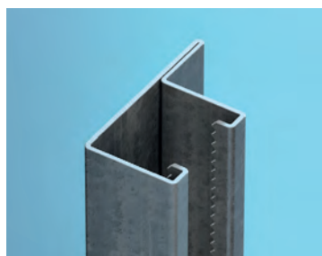
Ratchet track, inner, B 70 x T 37 mm 901201 (WP W03-02)
